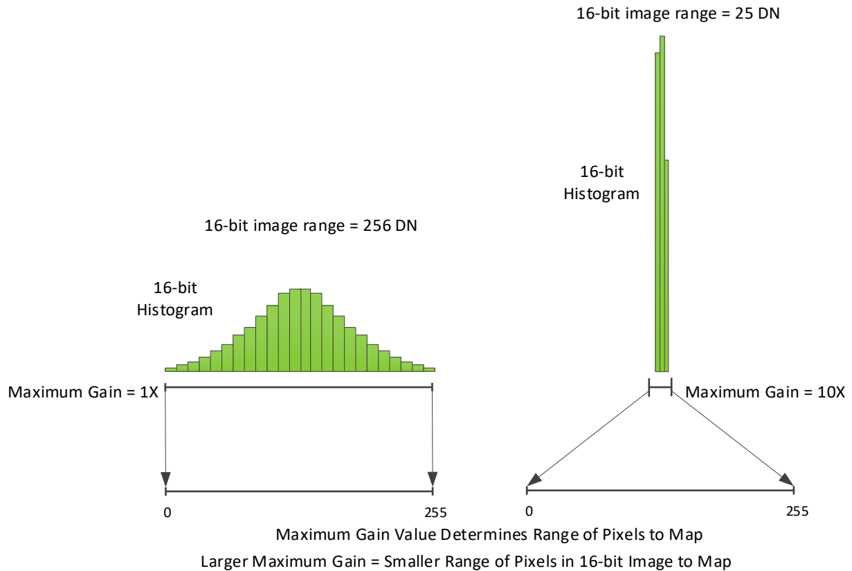
Figure 17: Contrast Enhancement Maximum Gain
