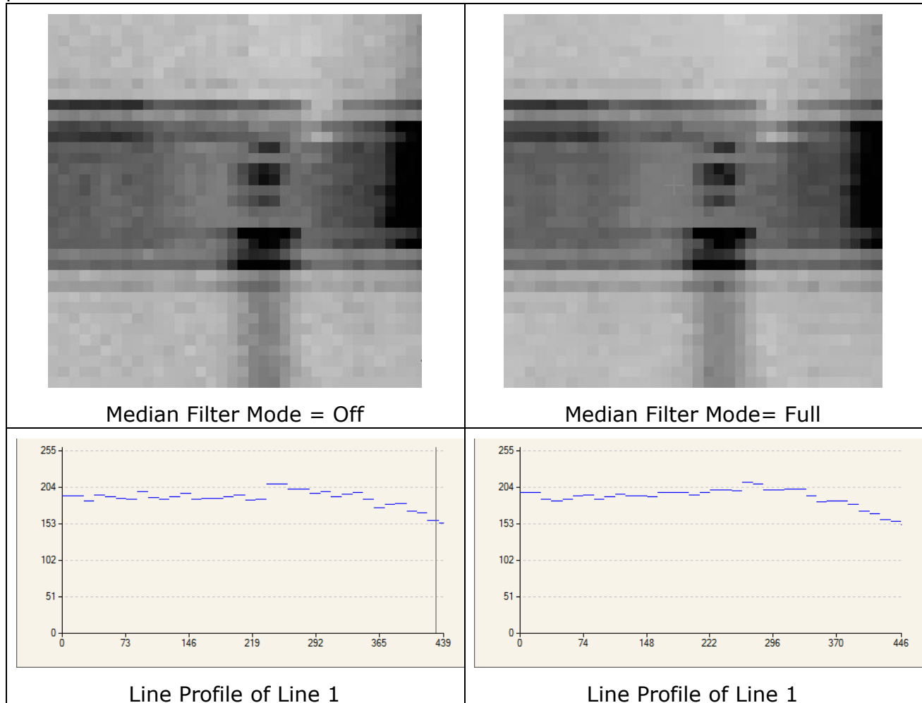
Figure 14: Median Filter
