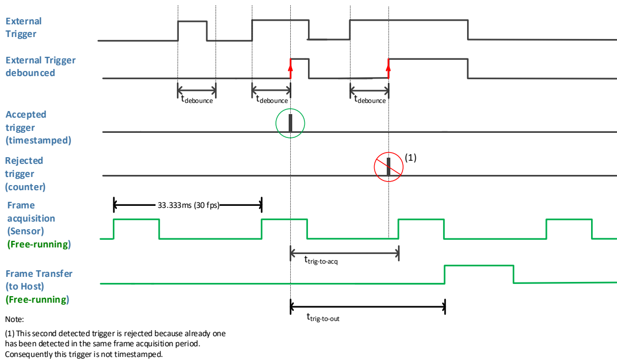
Figure 21: External Trigger Wave Diagram: Free-Running
