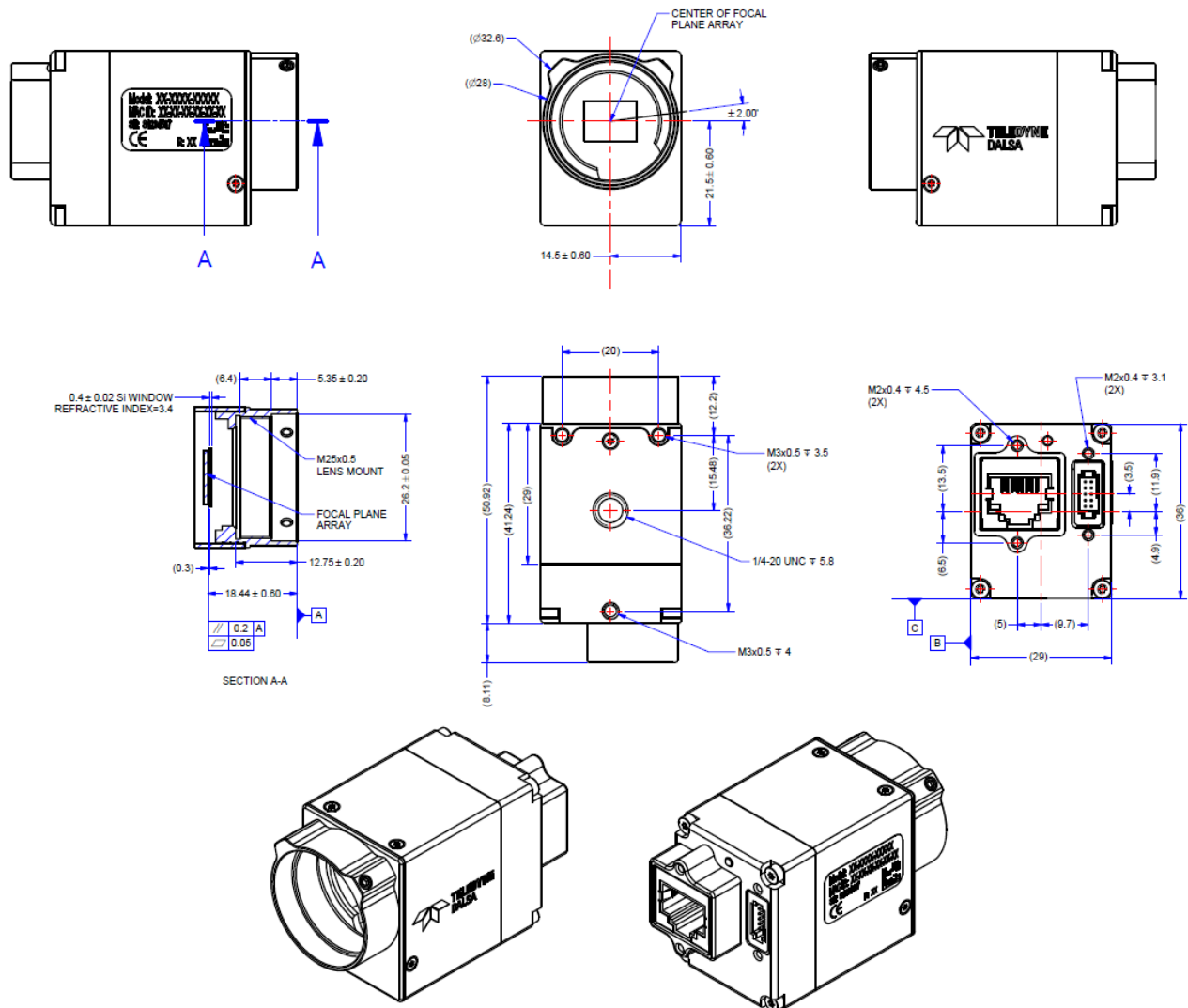
Figure 49: Calibir GXM640 with M25 Lens Mount (mm units)
