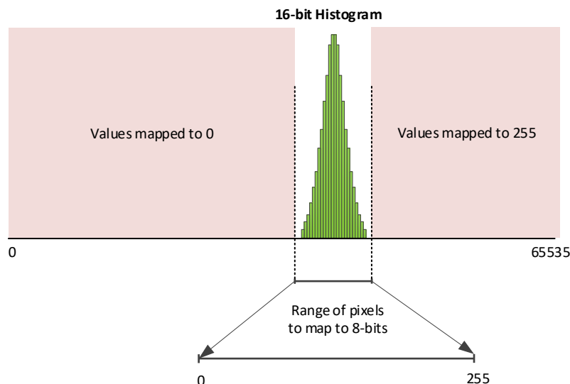
Figure 15: Contrast Enhancement Mapping 16-Bit to 8-bit
