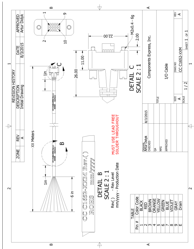
Figure 51: Cable Assembly G3-AIOC-BLUNT2M Mechanical Drawing
